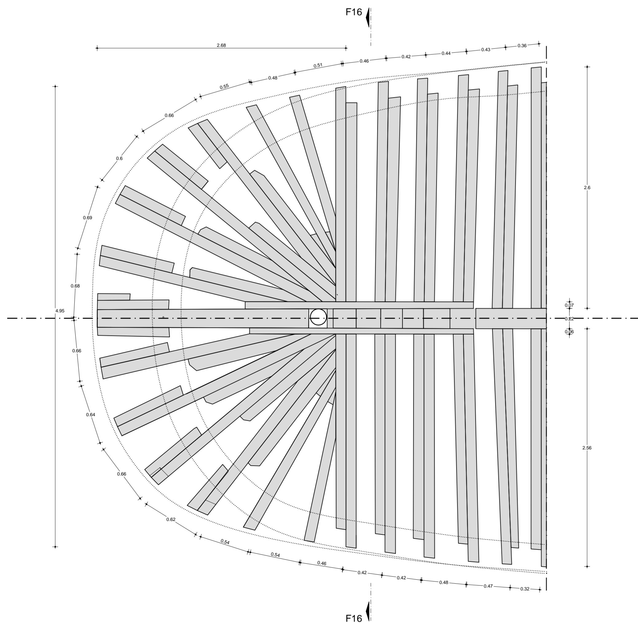
OVERHEAD PLAN OF FRAMES
