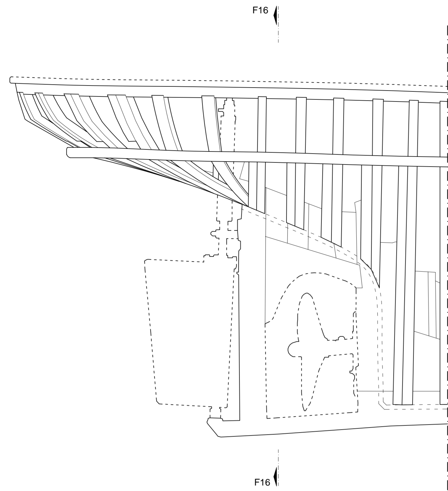
SIDE VIEW UNPLANKED
