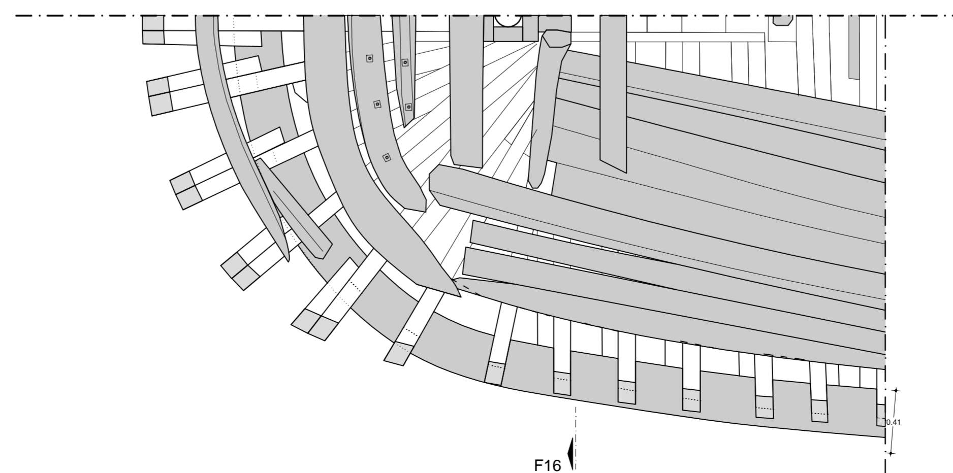
OVERHEAD PLAN OF LONGITUDINAL STRUCTURE
