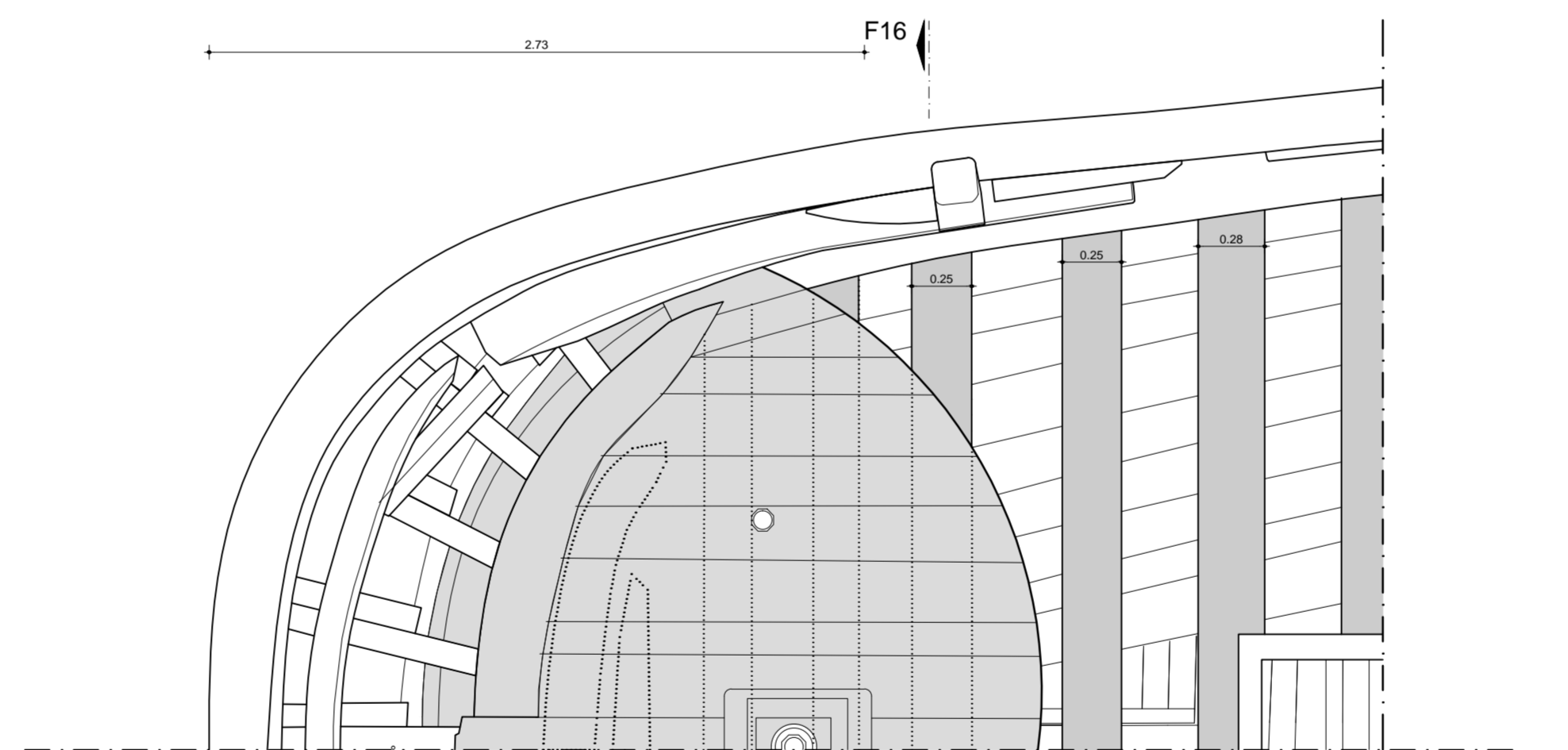
OVERHEAD PLAN OF BEAMS AND DECK
